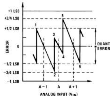
Figure 19. Clarifying the Error Specs of an ADC Converter Accuracy= \pm 1/4 LSB
