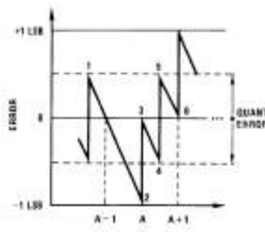
Figure 21. Clarifying the Error Specs of an ADC Converter Accuracy= \pm 1/2 LSB
