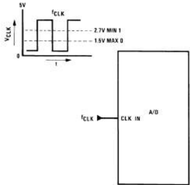
Figure 61. External clocking
